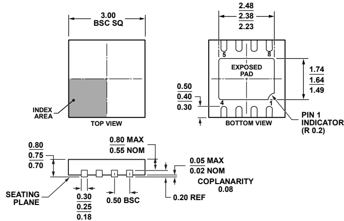
Figure 58. 8-Lead Lead Frame Chip Scale Package [LFCSP_WD] 3 mm x 3 mm Body, Very Very Thin, Dual Lead (CP-8-5)
