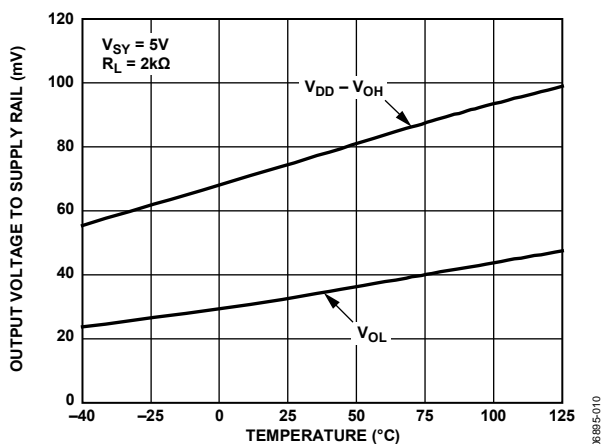
Figure 13. Output Voltage to Supply Rail vs. Temperature
